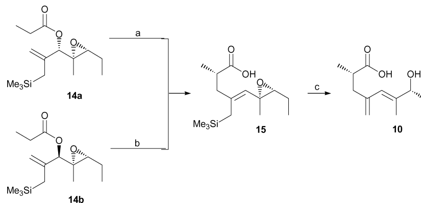
Scheme 4 Reagents and conditions: (a) LDA, THF, -78^\circ\text{C} , then TBSCl, DMPU; (b) LDA, THF, DMPU, -78^\circ\text{C} , then TBSCl; (c) \text{NH}_4\text{Cl} , \text{H}_2\text{O} , then HCl (2 M), 90%.
