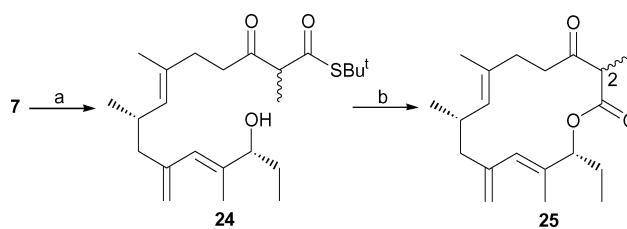
Scheme 10 Reagents and conditions: (a) \text{HOAc} - \text{H}_2\text{O} -THF, 2 : 2 : 1, 70%; (b) \text{Hg}(\text{OAc})_2 , \text{Pr}^i\text{NEt}_2 , THF, 99%.
