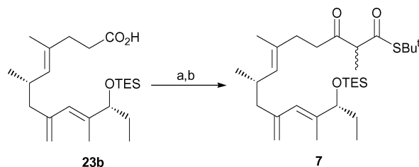
Scheme 9 Reagents and conditions: (a) CDI; (b) (\text{Bu}^t\text{SCOCH}(\text{CH}_3)_2\text{CO}_2)_2\text{Mg} , THF, 97%.
