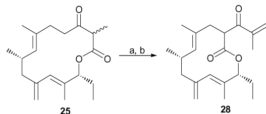
Scheme 12 Reagents and conditions: (a) LDA (10 eq.), THF, DMPU; (b) \text{H}_2\text{C}=\text{O} , THF, 39%.
