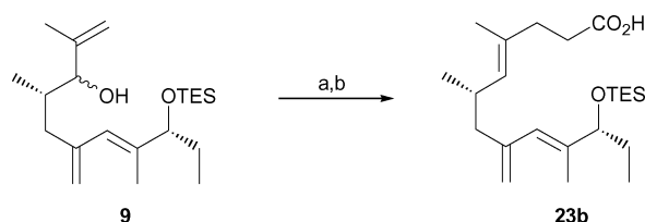
Scheme 8 Reagents and conditions: (a) \text{MeC}(\text{OEt})_3 , \text{C}_5\text{H}_{11}\text{CO}_2\text{H} ; (b) \text{KOH} - \text{EtOH} - \text{H}_2\text{O} , then \text{HCl} (0.1 M) 88%.
